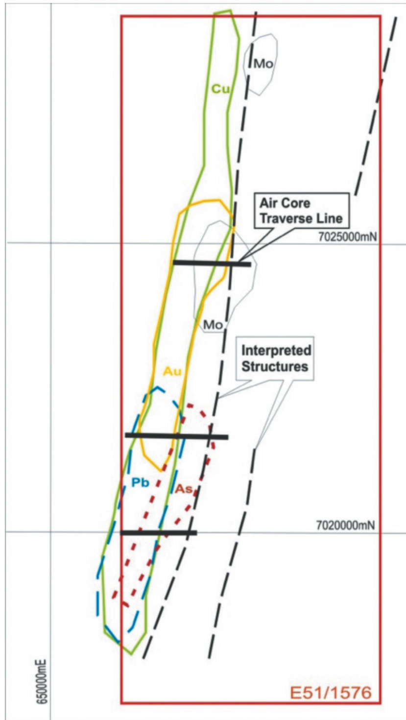
Figure 5 - Geochemical Contour Plot for Soil Au, Cu, Pb, As and Mo on E51/1576 from historical data by the Windy Knob Joint Venture Contours are areas above background levels for the listed elements.
