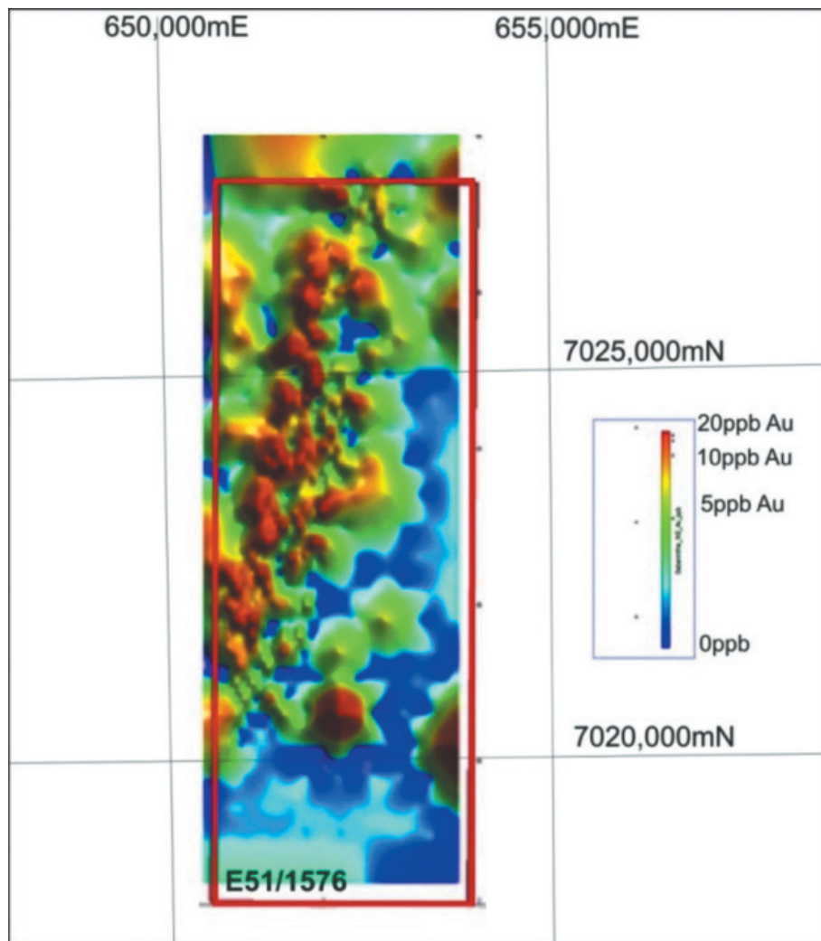
Figure 4 - Gold - in - Soil Geochemical anomalies on E51/1576.
