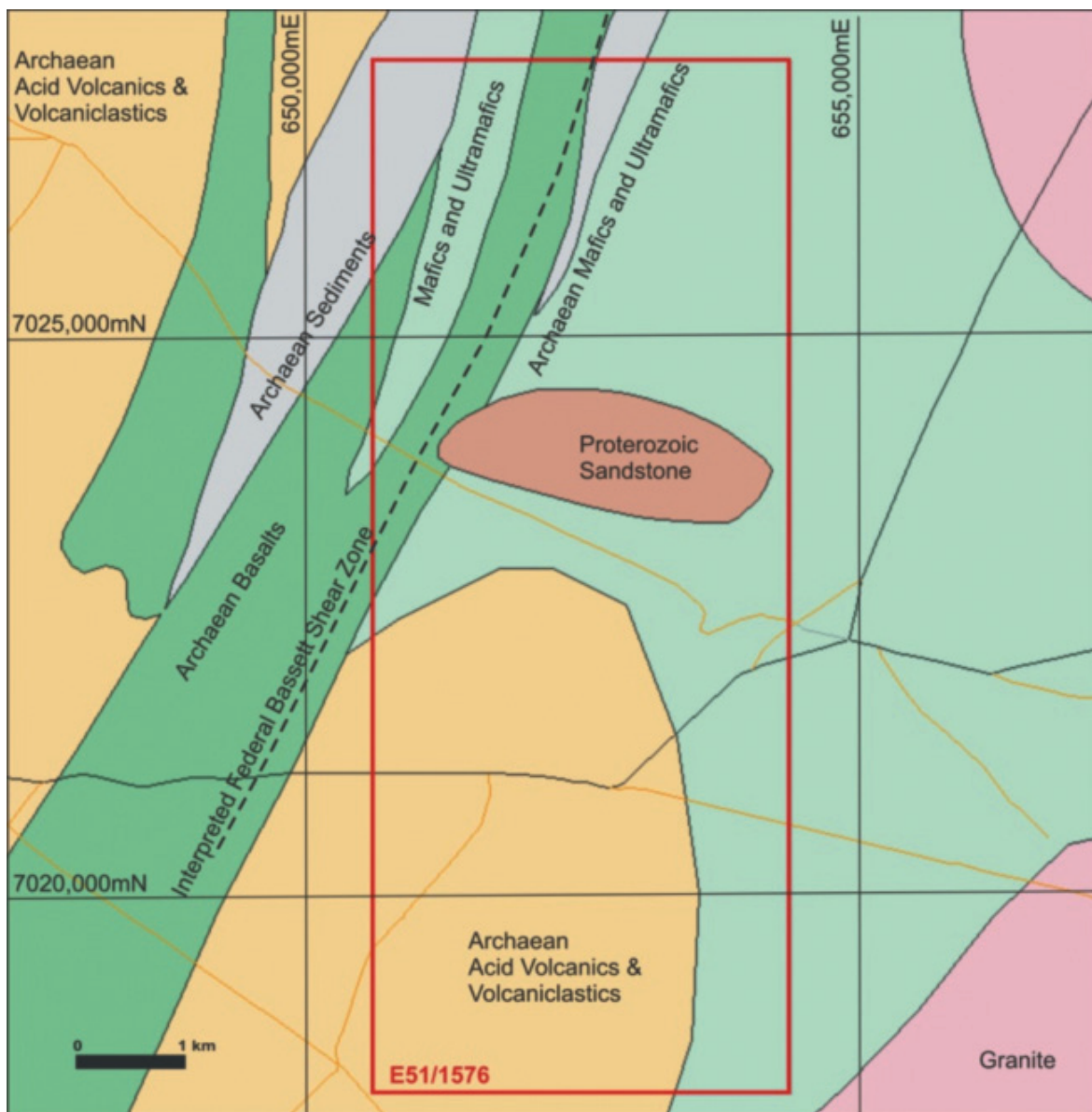
Figure 3 - Geological Setting of E51/1576.
